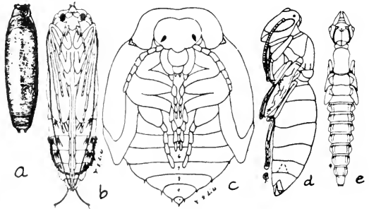
Fig. 72. a, Pupa of frit fly, Oscinella frit (L.); b, Pupa of Hesperophylax sp.; c, Pupa of Leptinotarsa decimlineata (Say); d, Pupa of Vespa maculata Kirby; e, Pupa of Corydalus cornutus (L.).
